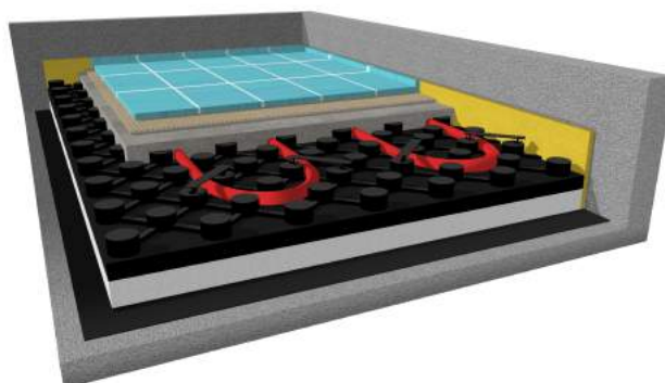
Płyta systemowa Profi System Duo Profi System Duo system board
